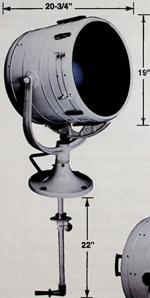
FIG. 1902 LEVER/GEAR CONTROL
