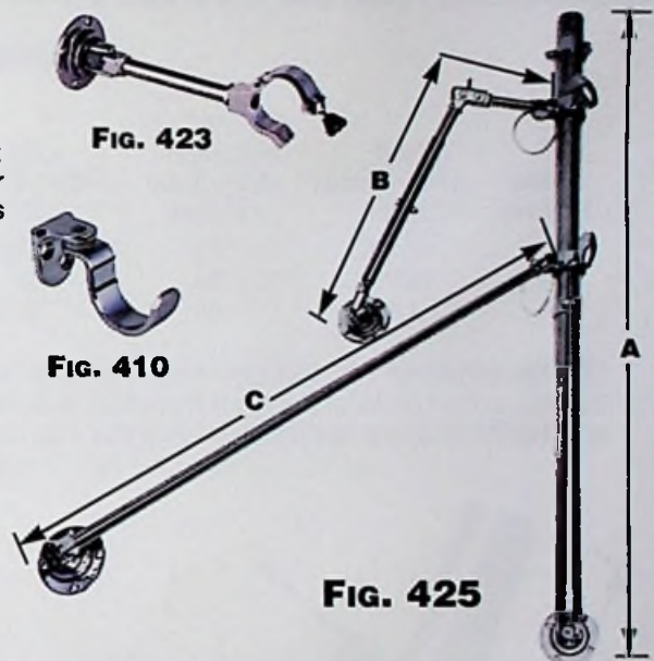
FIG. 400 - OUTRIGGER POLE HOLDERS
