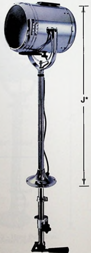
FIG. 884 HIGH PEDESTAL
