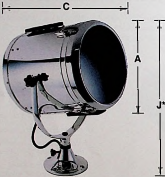
FIG. 883 - STANDARD PEDESTAL
