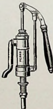
Fig. 479 With Straight Base
